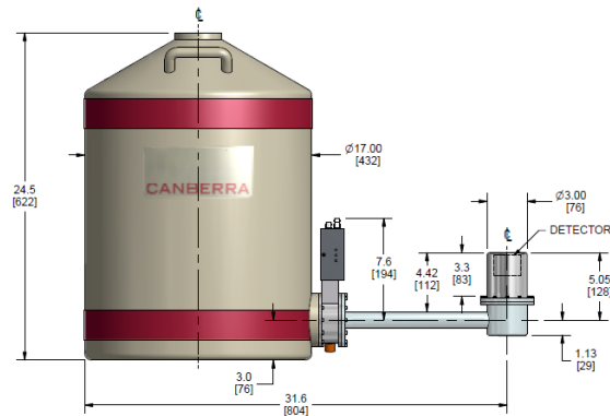
7905-30UM Horizontal Integral Cryostat (also available in 7.5 and 15 liter version)
