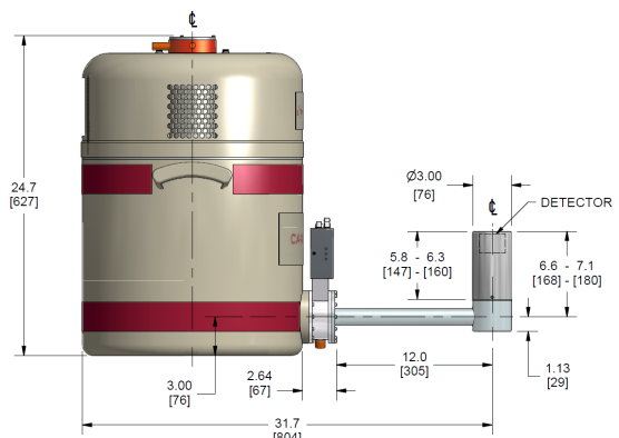
CCII-HI-U Horizontal Integral Hybrid Cryostat
